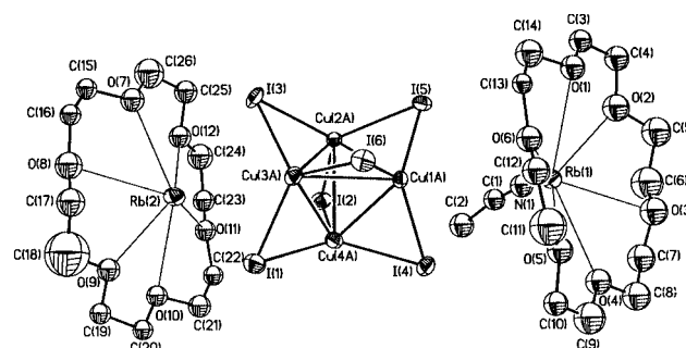
Fig. 1 Structure of [\{\text{Rb}(\text{18c6})\}_2\text{MeCN}][\text{Cu}_4\text{I}_6] \textbf{1} showing the hexa- \mu -iodo-tetrahedro-tetracuprate(I) anion sandwiched between the [\text{Rb}(\text{18c6})]^+ cations (the non-hydrogen atoms are shown as 20% thermal ellipsoids, H atoms omitted for clarity; only one of the two possible sets of the copper atoms is shown).
