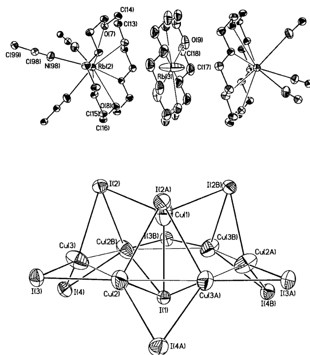
Fig. 3 View of [\text{Rb}(\text{18c6})(\text{MeCN})_3]^+ and [\text{Rb}(\text{18c6})]^+ cations and the [\text{Cu}_7\text{I}_{10}]^{3-} anion present in the crystal structure of complex 2 (the non-hydrogen atoms are shown as 30% thermal ellipsoids, H atoms omitted for clarity).
